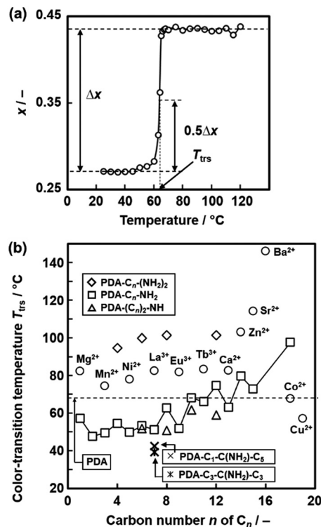
Fig. 12 Quantitative characterization of the color-transition temperature ( T_{tr} ). (a) Relationship between the temperature and x value of the PDA-C_8-NH_2 . 82 The x and \Delta x represent the intensity of the red color and the overall color change, respectively. The T_{tr} is defined as the temperature to achieve 0.5\Delta x . Reprinted with permission from Elsevier. 82 (b) Summary of the T_{tr} values of the layered PDA with intercalation of a variety of the guests. 79,82,83,85 Reprinted with permission from Wiley-VCH. 85
