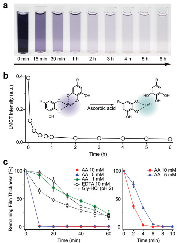
Fig. 1 (a) Time-lapse optical images of the \text{Fe}^{3+} -TA MPC solution after addition of ascorbic acid at 0 min (10 mM). (b) Graph of LMCT intensity at 565 nm versus reaction time. (c) Graphs of film thickness versus reaction time. The \text{Fe}^{3+} -TA MPC film was incubated in an aqueous solution of AA (1, 5, or 10 mM), EDTA (10 mM), or gly-HCl buffer (pH 2). The right graph for AA (5 and 10 mM) is the enlarged one for the first 10 min of incubation.
