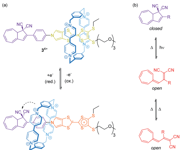
Fig. 4 (a) Redox-active [2]rotaxane 3^{4+} bearing a photo- and thermoswitchable dihydroazulene unit as stopper. The dashed arrow illustrates through-space interactions between \text{CBPQT}^{4+} wheel and dihydroazulene site. (b) Photo- and thermoswitching of the 1,1-dicyano-dihydroazulene moiety.
