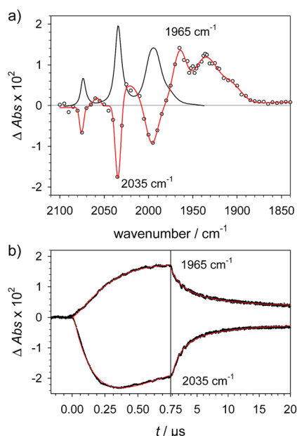
Fig. 2 (a) Transient IR spectrum 1\text{ }\mu\text{s} after excitation (O, \color{red}{\text{---}} ) and normalized IR spectrum of the starting state ( \text{---} ) for formation of \mathbf{1H} by protonation of \mathbf{1}^- with \text{Cl}_3\text{CCOOH} ( 13\text{ mM} ) following reduction of \mathbf{1} ( 1.3\text{ mM} ) by flash-quench generated [\text{Ru}(\text{dmb})_3]^+ in acetonitrile. (b) Kinetic traces ( \dots ) and fits ( \color{red}{\text{---}} ) monitoring pseudo-first order formation of \mathbf{1H} ( 1965\text{ cm}^{-1} ) and bleach of \mathbf{1} ( 2035\text{ cm}^{-1} ) followed by second order charge recombination with \text{TTF}^+ .
