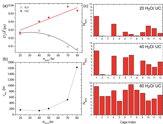
Fig. 24 (a) Self-diffusivities of water (empty symbols and dashed lines) and the center of excess charge (full symbols and solid lines) simulated at 400 K in UiO-66(Zr)-(CO 2 H) 2 as a function of water loading defined as the number of water molecules ( n_{H_2O} ) per unit cell (uc). (b) Residence time of water molecules in the cages of UiO-66(Zr)-(CO 2 H) 2 averaged over aMS-EVB3 trajectories obtained at 400 K as a function of water loading. (c) Simulated distribution of water in the tetrahedral (from 1 to 8) and octahedral (from 9 to 12) cages of UiO-66(Zr)-(CO 2 H) 2 at 400 K. Reproduced from ref. 84 with permission from American Chemical Society, Copyright 2017.
