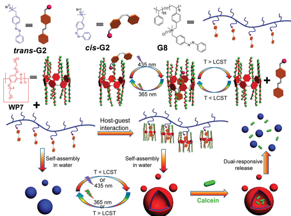
Fig. 7 Chemical structures of WP7, G2, and polymer G8, and cartoon representation of the controlled release process. Reproduced with permission from ref. 74. Copyright 2015, American Chemical Society.
