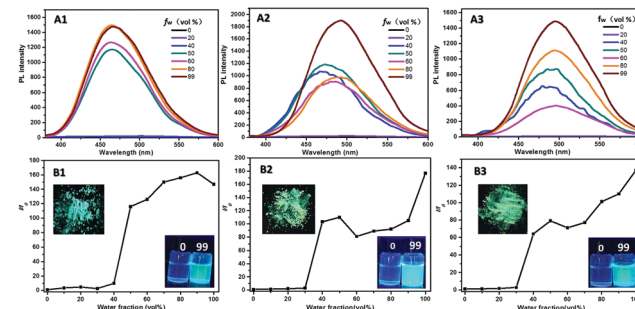
Fig. 3 Fluorescent spectra of TPE-L-Glu, cis -TPE-L-DGlu and trans -TPE-L-DGlu in THF/water mixed solvents with different f_w (A1–A3); plot of ||I_0 values versus f_w (B1–B3), where I_0 represents the emission intensity in THF. Concentration: 1 \times 10^{-5} M; excitation wavelength: 340 nm. Inset: Photographs of TPE-L-Glu, cis -TPE-L-DGlu and trans -TPE-L-DGlu in solid and THF/water mixtures with 0 and 99% f_w under 365 nm UV lamp.
