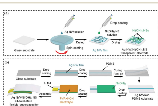
Scheme 1 Schematic of the fabrication of (a) the Ag NW/Ni(OH) 2 NS TE and (b) the all-solid-state flexible supercapacitor.
