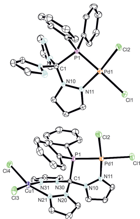
Fig. 5 Molecular structures of 7 and 8 . The thermal ellipsoids are at 30% probability level. Hydrogen atoms and solvent molecules ( 8 : acetonitrile) have been omitted for clarity. Selected bond lengths [pm] and angles [°]: 7 : \text{Pd1-P1} = 218.3(6) , \text{Pd1-Cl1} = 237.0(6) , \text{Pd1-Cl2} = 228.4(6) , \text{Pd1-N11} = 201.41(16) , \text{P1-C1} = 196.2(2) , \text{P1-Pd1-Cl1} = 175.411(19) , \text{P1-Pd1-Cl2} = 87.87(2) , \text{Cl2-Pd1-Cl1} = 94.91(2) , \text{N11-Pd1-P1} = 84.8 , \text{N11-Pd1-Cl1} = 92.31(5) , \text{N11-Pd1-Cl2} = 172.22(5) . 8 : \text{Pd1-P1} = 219.56(17) , \text{Pd1-Cl1} = 236.21(17) , \text{Pd1-Cl2} = 227.67(18) , \text{Pd1-N11} = 200.5(5) , \text{Cl1-Cl3} = 221.46(19) , \text{Cu1-N21} = 202.6(5) , \text{Cu1-N31} = 201.4(5) , \text{P1-C1} = 195.2(6) , \text{Pd1...Cu1} = 603.61(14) , \text{P1-Pd1-Cl1} = 172.30(6) , \text{P1-Pd1-Cl2} = 87.97(7) , \text{Cl2-Pd1-Cl1} = 94.47(7) , \text{N11-Pd1-P1} = 84.84(15) , \text{N11-Pd1-Cl1} = 92.67(15) , \text{N11-Pd1-Cl2} = 172.81(15) , \text{Cl3-Cu1-Cl4} = 94.63(8) , \text{N21-Cu1-Cl3} = 91.32(15) , \text{N21-Cu1-Cl4} = 161.49(15) , \text{N31-Cu1-N21} = 84.8(2) , \text{N31-Cu1-Cl4} = 90.07(15) , \text{N31-Cu1-Cl3} = 174.86(15) .
