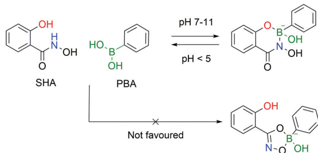
Fig. 24 Complexation of SHA with PBA occurs readily at neutral and alkaline pHs but the formed complex is quickly hydrolysed under acidic conditions. The 6-membered ring is the preferential structure.
