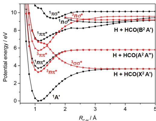
Fig. 3 Rigid body singlet (in black) and triplet (in red) PECs for HCHO plotted as a function of R_{\text{C}-\text{H}} for planar geometries, with the rest of the nuclear framework maintained at its ground state equilibrium geometry.
