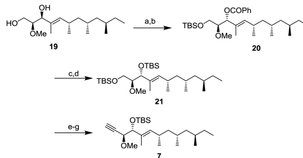
Scheme 4 Synthesis of alkyne 7 ; (a) TBSCl, imidazole, \text{CH}_2\text{Cl}_2 , r.t., 2 h, 81%; (b) \text{PhCOOH} , DEAD, \text{PPh}_3 , THF, r.t., 15 h, 95%; (c) \text{K}_2\text{CO}_3 , \text{MeOH} , r.t., 12 h; (d) \text{TBSOTf} , 2,6-lutidine, \text{CH}_2\text{Cl}_2 , -78 °C, 2 h, 98% (2 steps); (e) PPTS, \text{EtOH} , r.t., 16 h, 80%; (f) DMP, \text{CH}_2\text{Cl}_2 , r.t., 2 h; and (g) dimethyl(1-diazo-2-oxopropyl)phosphonate, \text{K}_2\text{CO}_3 , \text{MeOH} , r.t., 18 h, 58% (2 steps).
