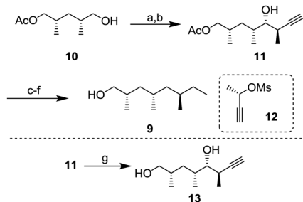
Scheme 2 Synthesis of alcohol 9 ; (a) IBX, DMSO, r.t., 3 h, 85%; (b) 12 , \text{Pd}(\text{OAc})_2 , \text{PPh}_3 , \text{ZnEt}_2 , THF, -78 °C to -20 °C, 6 h, 70%; (c) \text{Pd/C} , \text{H}_2 , \text{MeOH} , r.t., 18 h, 85%; (d) phenyl chlorothionoformate, DMAP, pyridine, \text{CH}_2\text{Cl}_2 , r.t., 3.5 h, 74%; (e) n\text{Bu}_3\text{SnH} , AIBN, toluene, 100 °C, 16 h; (f) \text{K}_2\text{CO}_3 , \text{MeOH} , r.t., 2 h, 96% (2 steps); and (g) \text{K}_2\text{CO}_3 , \text{MeOH} , r.t., 3 h, 85%.
