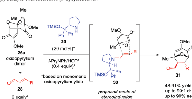
Scheme 6 [5+2] Cycloaddition of oxidopyrylium dimer 26 by Murelli and Brenner-Moyer.
