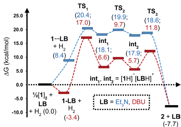
Fig. 5 Computed free energy profile for Et 3 N- and DBU-assisted H 2 activation with 1 . Relative free energies (in kcal mol -1 ) are with respect to \frac{1}{2}[\mathbf{1}]_2 + \text{LB} + \text{H}_2 .
