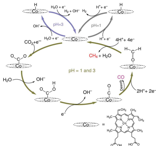
Scheme 12 Catalytic cycle for two electron reduction of \text{CO}_2 to \text{CO} and further reduction to \text{CH}_4 with a \text{CoPP} protoporphyrin molecular catalyst ( \text{CoPP} ) immobilized onto a pyrolytic graphite ( \text{PG} ) electrode ( \text{CoPP-PG} ). Reprinted with permission from ref. 147. Copyright 2015, Nature Publishing Group.
