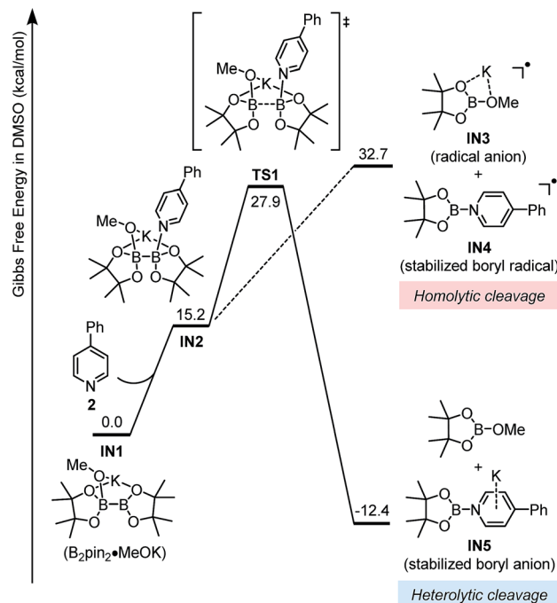
Fig. 5 Gibbs free energy ( \Delta G_{\text{solvent}}^{\ddagger} ) profile for the homolytic and heterolytic cleavage pathways of diboron.
