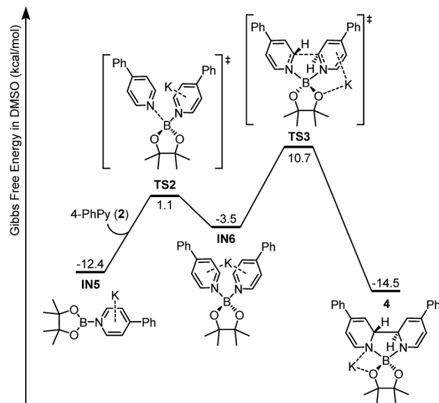
Fig. 6 Gibbs free energy ( \Delta G_{\text{solvent}}^{\ddagger} ) profile for the formation of ate complex 4 .
