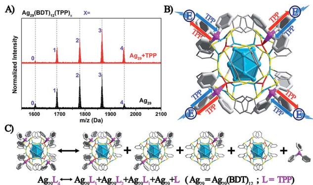
Fig. 3 (A) ESI-MS spectra of the Ag_{29}(BDT)_{12}(TPP)_4 NC with or without the addition of TPP. (B) Illustration of the dynamic TPP dissociation–aggregation process on the Ag_{29}(BDT)_{12}(TPP)_4 and the corresponding energy loss. (C) The dynamic TPP dissociation–aggregation reversible reaction. Color codes: cerulean/red spheres, Ag; yellow spheres, S; purple spheres, P; grey spheres, C; white spheres, H.
