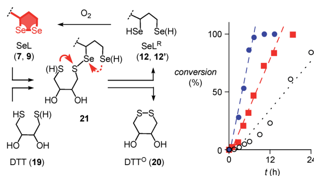
Fig. 4 Oxidation of 500 \mu\text{M} 19 to 20 as a function of time in the absence (○) and the presence of 500 \mu\text{M} 9 (■) and 22 (●) in \text{D}_2\text{O} , \text{pD} = 8.0 , with linear fits to determine the t_{50} . Structures are shown in neutral form, acidic protons are indicated in parenthesis. Competing ring closures in reactive intermediate 21 are indicated with solid (preferred) and dashed red arrows.
