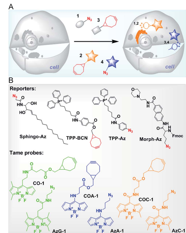
Fig. 1 (A) A schematic illustration of multi-color intracellular labelling in live cells via SPAAC. Azide- and cyclooctyne-containing reporters (1 and 3) can be ligated with cyclooctyne- and azide-containing probes (2 and 4), respectively, at specific sites of the cells. Firstly, cells pre-treated with reporter 1 are incubated with probe 2 to target the first organelle. After a brief wash, a second reporter 3 is introduced into cells followed by labelling with probe 4 to label the second organelle. The unreacted probe is then washed out of the cells. (B) The structures of reporters to target Golgi apparatus ( Sphingo-Az ), mitochondria ( TPP-BCN and TPP-Az ) and lysosome ( Morph-Az ) in addition to the tame probes: green CO-1 and AzG-1 , blue COA-1 and AzA-1 , and yellow COC-1 and AzC-1 .
