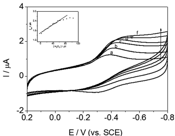
Fig. 11 Cyclic voltammograms of DM-EB/Hb/GCE with (a) 0 μmol L -1 , (b) 3.5 μmol L -1 , (c) 24.5 μmol L -1 , (d) 31.5 μmol L -1 , (e) 63.0 μmol L -1 and (f) 84.0 μmol L -1 H 2 O 2 in PBS (pH 7.0), and plots of the electrocatalytic current ( I_{cat} ) vs. H 2 O 2 concentration on DM-EB/Hb/GCE (inset). Scanning rate, 200 mV s -1 .
