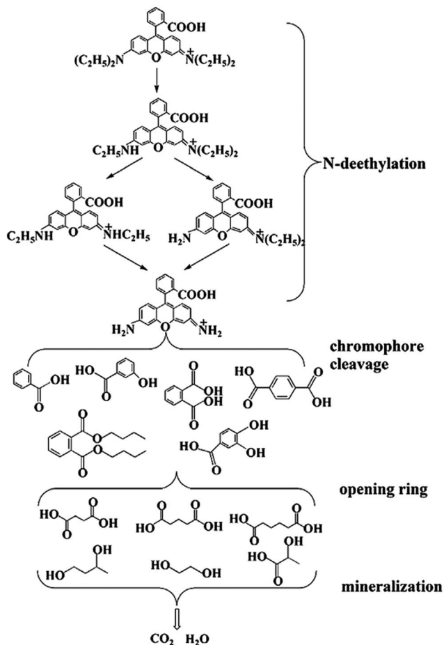
Fig. 13 The possible degradation intermediate and the final products of RhB over BiOI/Ag 2 CO 3 composites.
