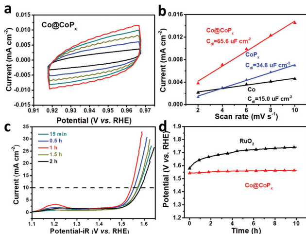
Fig. 5 (a) Cyclic voltammety curves of \text{Co@CoP}_x in the region where no redox reaction occurs; the scan rates are 10, 8, 6, 4, and 2 \text{mV s}^{-1} . (b) Current density as a function of the scan rate for the Co nanochains, \text{CoP}_x and \text{Co@CoP}_x nanochains. (c) Polarization curves of the samples prepared under different phosphorization times. (d) Chronopotentiometry curves of \text{Co@CoP}_x and \text{RuO}_2 .
