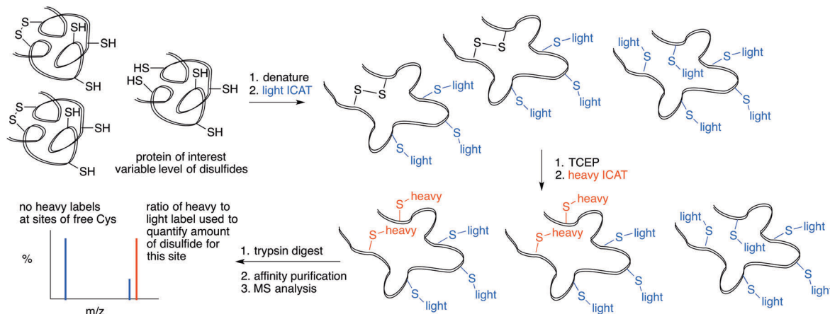
b) ICAT analysis can be used to identify and quantify levels of disulfide vs thiol for specific cysteines
