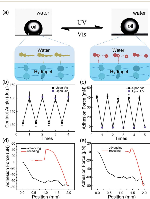
Fig. 4 Underwater photo-responsive properties of the IBSP-modified hydrogel. (a) In an underwater environment, the oil (1,2-dichloroethane, 2 \mu\text{L} ) contact angle (OCA) on the IBSP-modified hydrogel can be reversibly switched by UV (365 nm, 120 \text{mW cm}^{-2} , 20 s) and Vis (470 nm, 30 \text{mW cm}^{-2} , 10 min) illumination. (b) Photo-responsive reversible switch of the underwater OCA on the IBSP-modified hydrogel. (c) Photo-responsive reversible switch of the underwater oil (5 \mu\text{L} ) adhesion force on the IBSP-modified hydrogel. Force–distance curves during the underwater oil adhesion force measurements (d) before and (e) after UV irradiation.
