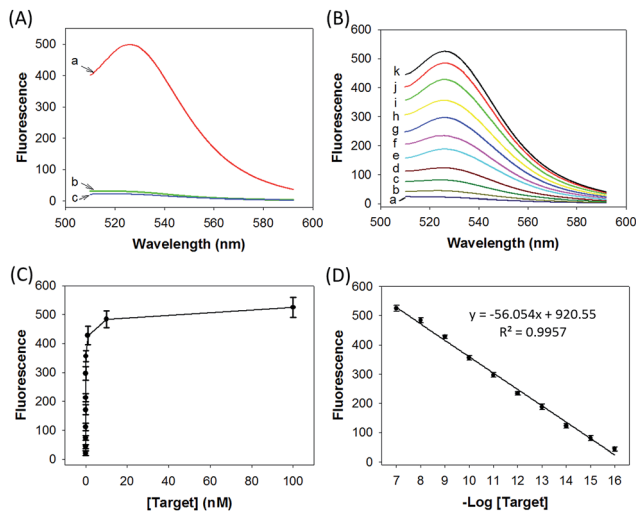
Fig. 2 (A) Fluorescence spectra obtained by incubating the nano-system carrying H0, H1, H2 and H3 with the (a) target sequence, (b) nontarget sequence, and (c) assay buffer as well as the target sequence. (B) Fluorescence spectral responses to the target sequence with different concentrations: (a) 0 M, (b) 1 \times 10^{-16} M, (c) 1 \times 10^{-15} M, (d) 1 \times 10^{-14} M, (e) 1 \times 10^{-13} M, (f) 1 \times 10^{-12} M, (g) 1 \times 10^{-11} M, (h) 1 \times 10^{-10} M, (i) 1 \times 10^{-9} M, (j) 1 \times 10^{-8} M, and (k) 1 \times 10^{-7} M target sequence. (C) Plot of fluorescence peak intensities (at 526 nm) versus target concentrations. (D) Fluorescence peak intensities versus target concentrations on a logarithmic scale.
