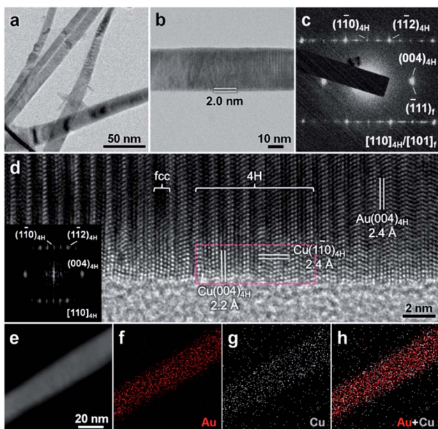
Fig. 4 (a) Low-magnification TEM image of alternating 4H/fcc bimetallic Au@Cu core-shell NRBs. (b) High-magnification TEM image and (c) corresponding SAED pattern of a representative Au@Cu NRB. (d) A representative HRTEM image of Au@Cu NRBs. Inset: the corresponding FFT pattern of the selected region, i.e. the magenta dashed rectangle in (d). (e) HAADF-STEM image, and (f–h) corresponding STEM-EDS element maps of a representative Au@Cu NRB.
