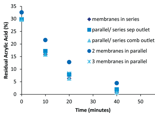
Fig. 3 Influence of reactor design on separation, the determination of residual monomer was performed by 1 H NMR analysis.
