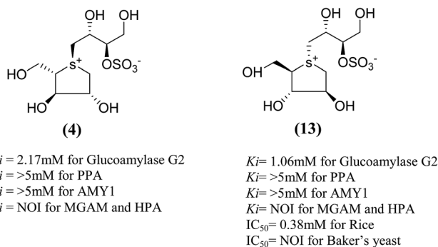
Fig. 6 Stereoisomers of salacinol (4 and 13) and their inhibitory activity against \alpha -glucosidases.
