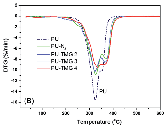
Fig. 7 TGA (A) and DTG (B) curves of PU, PU- \text{N}_3 , PU-TMG 2 (wt% = 1.0%), PU-TMG 3 (wt% = 2.1%), and PU-TMG 4 (wt% = 5.5%) under nitrogen.
