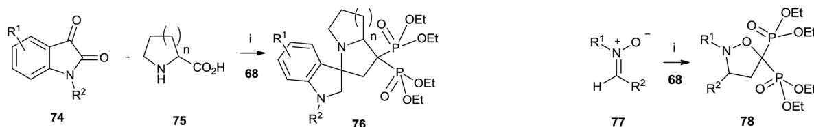
Scheme 18 Reagents and conditions: (i) Cu(OTf) 2 (10 mol%), toluene, 18 h, 70 °C. (ii) TMSBr, 18 h, rt; then water, 4 h, rt.
