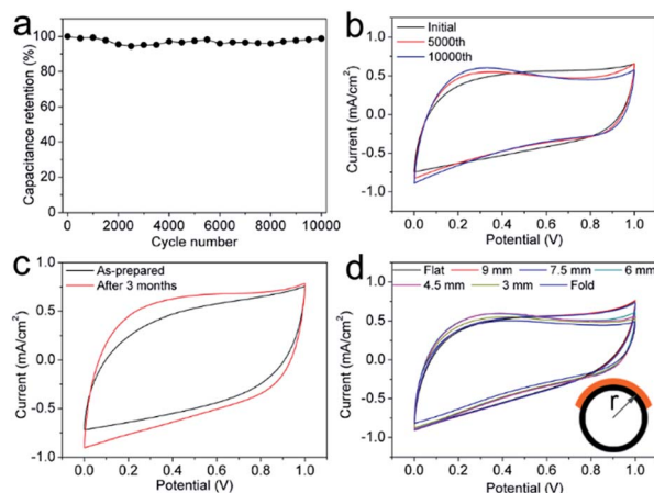
Fig. 5 (a) Cycling stability at a scan rate of 50 \text{ mV s}^{-1} , (b) CV curves of the initial, 5000th, and 10000th cycles, (c) CV curves of the as-prepared C/ \text{TiO}_2 MSC and the MSC after 3 months (scan rate 50 \text{ mV s}^{-1} ), and (d) CV curves of MSCs bent with different curvature radii (scan rate 50 \text{ mV s}^{-1} ). Inset in (d) is a schematic picture of a single MSC bent at different curvature radii.
