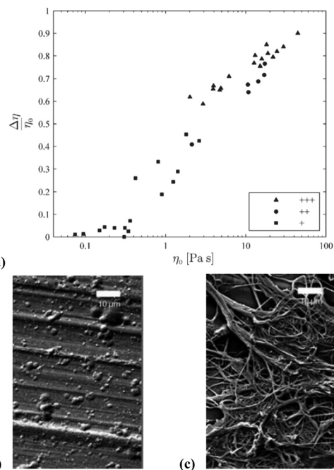
Fig. 12 (a) Relationship between shear thinning of OES–cellulose mixtures, and the propensity for fibre formation: + denotes no fibre formation; ++ denotes partial fibre formation; +++ denotes good fibre formation. Scanning Electron Microscopy (SEM) images for example ‘+’ and ‘+++’ cellulose electrospinning experiments are shown in (b) and (c), respectively (scale bars denote 10 μm). Reproduced and adapted with permission from J. Appl. Polym. Sci. , 2012, 125 , 1901–1909. Wiley-VCH Verlag GmbH & Co. KGaA, 2012.
