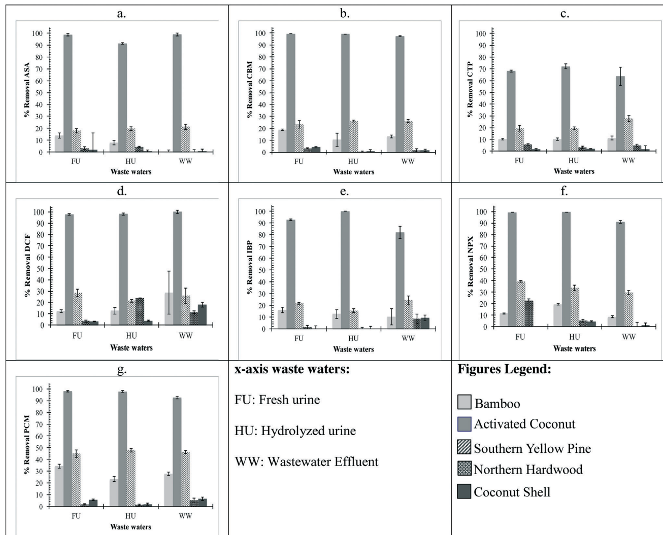
Fig. 2 Pharmaceutical removal by biochar at 0.8 g L -1 dose and 300 rpm for 24 h (C 0 = 0.2 mmol L -1 ). Pharmaceuticals: a. ASA, b. CBM, c. CTP, d. DCF, e. IBP, f. NPX, and g. PCM. Error bars indicate one standard deviation for triplicate samples.
