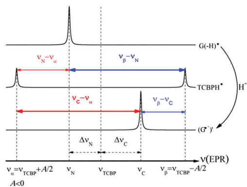
Scheme 1 Schematic representation of triplet-singlet interconversion based on the EPR spectra of \text{G}(\text{H})^{\bullet} (top), \text{TCBPH}^{\bullet} (middle), and (\text{G}^{\bullet+})' (bottom). Only a single spin-1/2 nucleus in \text{TCBPH}^{\bullet} with negative HFCC is considered.
