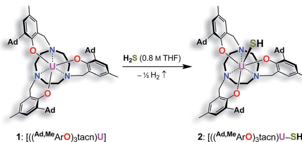
Scheme 1 Synthesis of the uranium(IV) hydrosulfido complex [[(\text{ArO})_3\text{tacn}]\text{U}-\text{SH}] ( 2 ).
