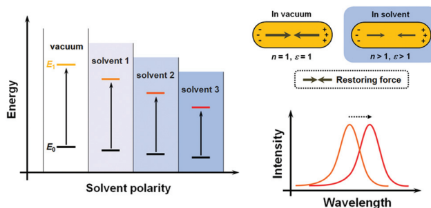
Fig. 1 Comparison of the mechanisms of solvatochromism of organic dyes and plasmonic nanostructures. (Left) Energy diagram of dye molecules in different solvents. (Right) Schematic illustration of (top) variation of the restoring force and (bottom) shifting of the plasmonic peak in different environments.
