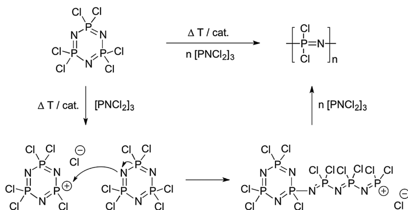
Fig. 5 Thermally and/or catalytically induced ring opening polymerisation representing the classical route to synthesise poly(dichloro)phosphazene [\text{N}(\text{P}(\text{Cl}_2)_2)_n] and its commonly accepted mechanism.
