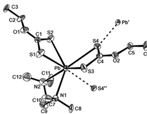
Fig. 12 The asymmetric unit of [\text{Pb}(\text{S}_2\text{COEt})_2\text{-tmeda}] showing the labelling scheme used; thermal ellipsoids are at the 40% level. Reproduced from ref. 104 with permission from The Royal Society of Chemistry.
