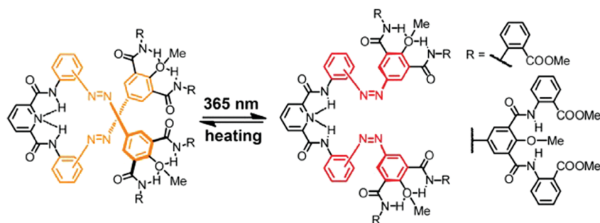
Fig. 9 Photoswitchable folded dendrons composed of a pyridine-2,6-dicarboxamide focal point and 2-methoxyisophtalamide termini connected via azobenzene units. 93
