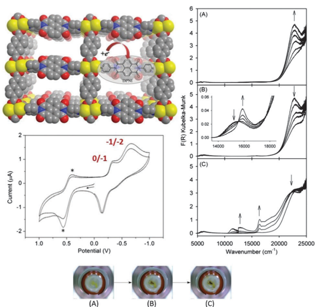
Fig. 2 Solid state electrochemistry and vis/NIR spectroelectrochemistry of [Zn 2 (ndc) 2 (DPNI)]. Cyclic voltammetry reveals two redox waves corresponding to generation of the radical anion and dianion states of the redox-active DPNI ligand. The optical properties of these states can be rapidly accessed using spectroelectrochemistry for generation of the radical anion (A) and dianion (B) states, which are accompanied by marked colour changes as seen in the photographs of the MOF on the transparent working electrode (bottom). Application of a more reducing potential leads to framework degradation (C). Reproduced from ref. 9 with permission from the Royal Society of Chemistry.
