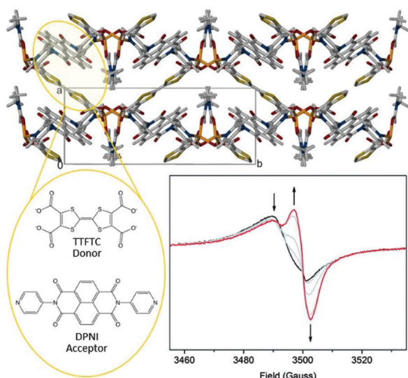
Fig. 3 The charge transfer MOF [(Zn(DMF)) 2 (TTFTC)(DPNI)] which exhibits through-space CT interactions. Reduction of the MOF switches the CT off. This is consistent with solid state EPR spectroelectrochemistry which revealed evidence for a concomitant decrease in the TTFTC radical cation, and an increase in the DPNI radical anion signal, thus reducing the donor-acceptor interaction. Reproduced from ref. 62 with permission from the Royal Society of Chemistry.
