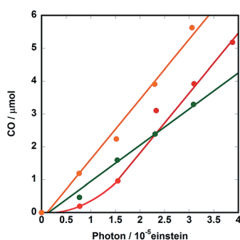
Fig. 8 Photocatalytic CO formation using DMF-TEOA (5:1 v/v) solutions containing 0.1 M of BNAH and 0.3 mM of Ru(CH 2 OCH 2 )Re (red), Ru(CH 2 OCH 2 )Re(CO) 3 (X) (green), or a 3:1 mixture of Ru(CH 2 OCH 2 )Re and Ru(CH 2 OCH 2 )Re(CO) 3 (X) (orange). The reaction conditions were same as those described in Fig. 5.
