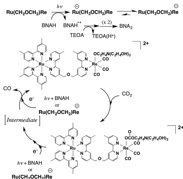
Scheme 1 Partial reaction mechanism of photocatalytic CO 2 reduction by Ru(CH 2 OCH 2 )Re.
