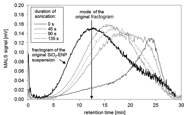
Fig. 3 Effect of increasing time of sonication after particle stabilisation in 0.025% FL-70™ and pH adjustment on AF 4 fractrogram.
