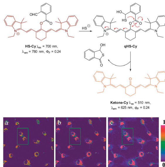
Fig. 52 Top: structure and reaction of HS-Cy with HS - . Bottom: confocal fluorescence ratiometric images of endogenous HS - in living A549 cells. A549 cells loaded with 5 mM HS-Cy for 30 min (a). Cells were pre-stimulated with SNP, then incubated with HS-Cy for 10 min (b) and 20 min (c). Scale = 50 nm. Image reproduced with permission. 222
