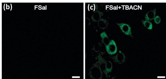
Fig. 27 Top: structure and reaction of fluorene based FSal with \text{CN}^- . Bottom: images of SH-SY5Y neuronal cells which were incubated with (left) FSal alone and (right) FSal then TBACN. Image reproduced with permission. 173
