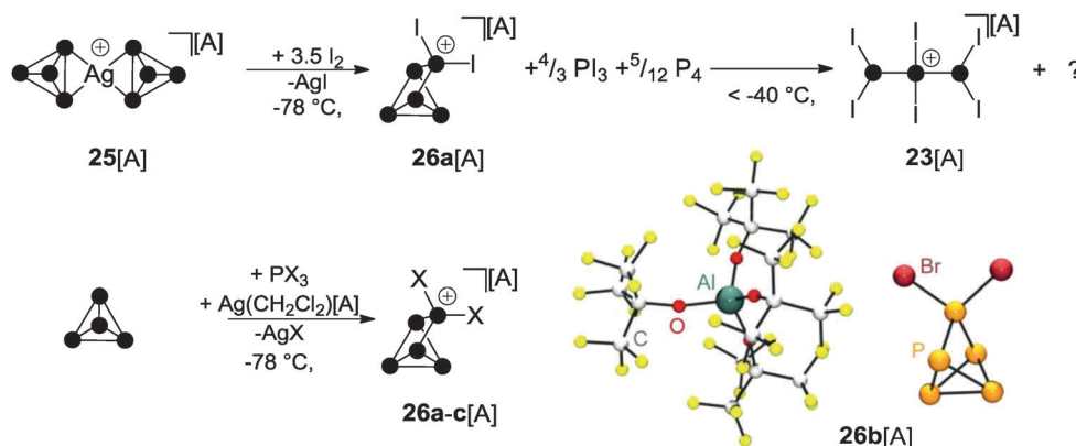
Scheme 7 Oxidation of Ag(I) complex 25[A] with I 2 at low temperatures giving intermediary P 5 I 2 + -cage 26a + (top), targeted syntheses of P 5 X 2 + -cages 26a-c + (X = I, Br, Cl) by the reaction of P 4 , PX 3 and Ag(CH 2 Cl 2 )[A] and molecular structure of 26b + (bottom); A = Al(OC(CF 3 ) 3 ) 4 .
