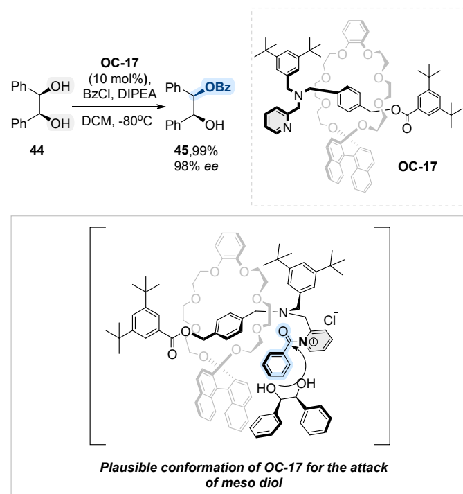
Scheme 27. Rotaxane-based catalyst ( OC-17 ) for asymmetric regioselective benzylation of meso -1,2-diol.
