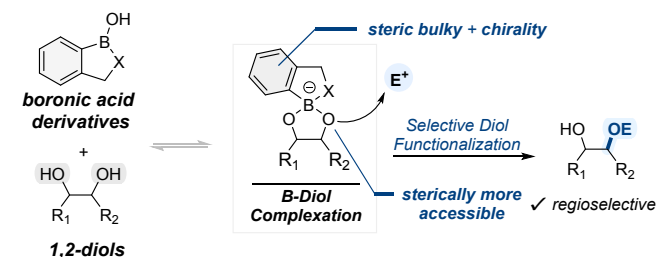
Scheme 17 General mechanism for heterocyclic boronic acid-catalyzed selective functionalization of diols.
