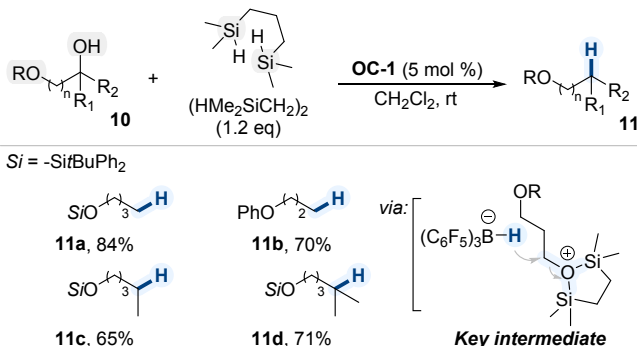
Scheme 7. BCF-catalyzed chemoselective deoxygenation of naked hydroxyl group in diols containing diverse ether functionalities.
