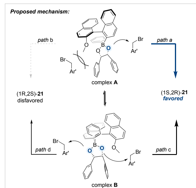
Scheme 13. Alkylative desymmetrization of 1,2-diols catalyzed by chiral borinic acid.
