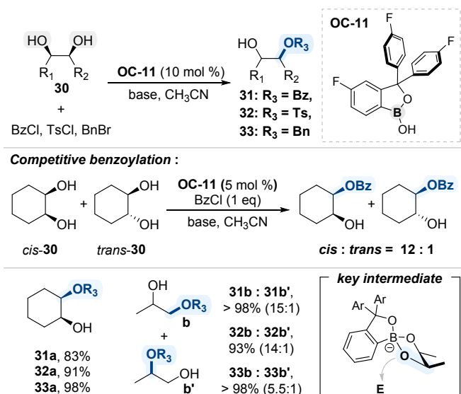
Scheme 20. Site-selective modification of diols catalyzed by OC-11 .
