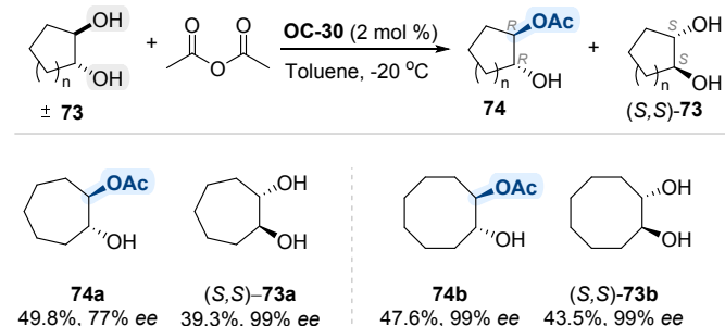
Scheme 42. Kinetic resolution of trans -cycloalkane-1,2-diols employing OC-30 .
