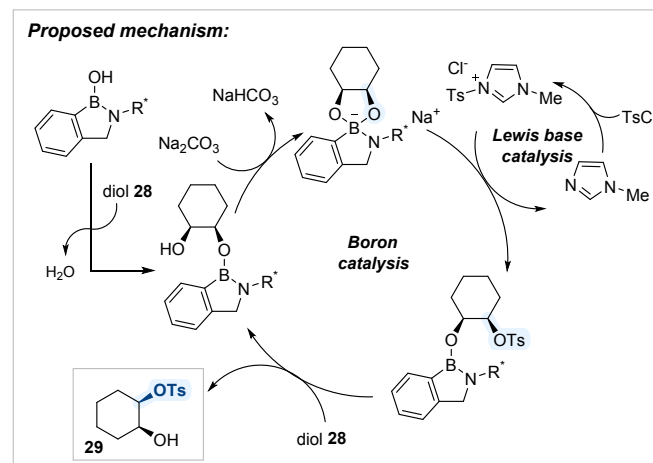
Scheme 19. Chiral benzazaborole-catalyzed enantioselective sulfonylation of meso -1,2-diols.
