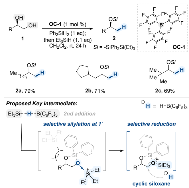
Scheme 3. BCF-catalyzed regioselective deoxygenation of terminal 1,2-diols.
