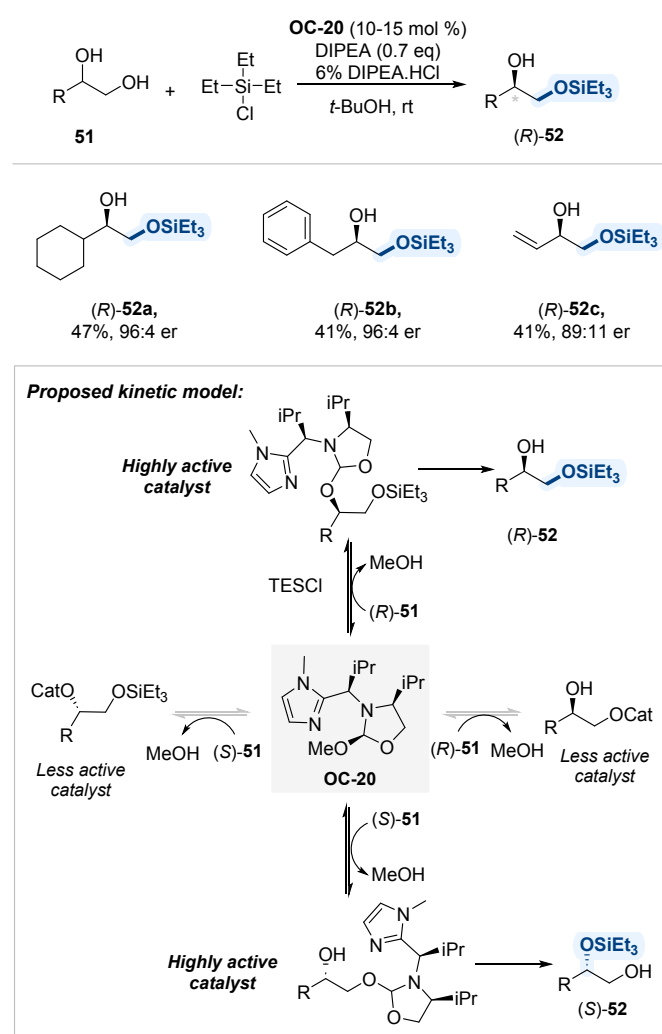
Scheme 30. Regiodivergent kinetic resolution of terminal 1,2-diols.
