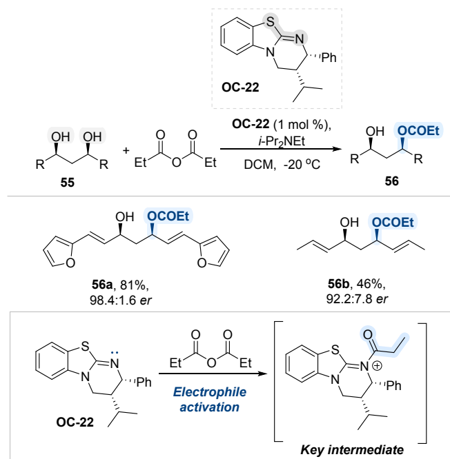
Scheme 32. Isothiourea catalyzed desymmetrization of meso 1,3-diols.
