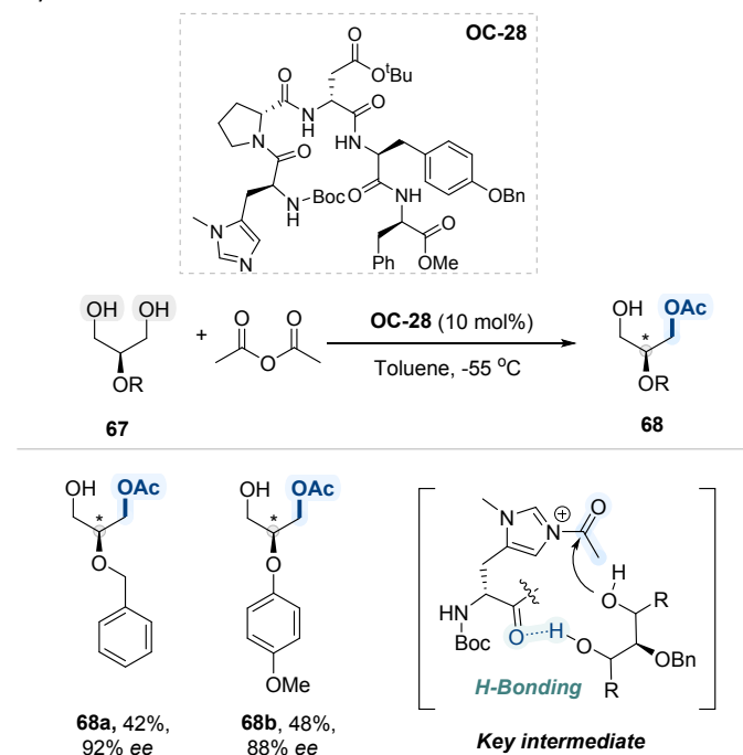
Scheme 39. Selective acylation of glycerol derivatives.
