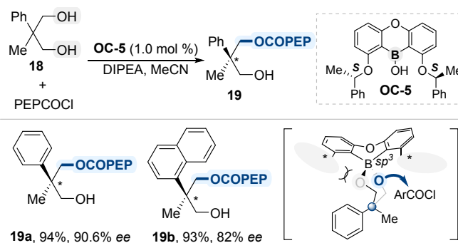
Scheme 12. Asymmetric desymmetrization using chiral borinic acid.
