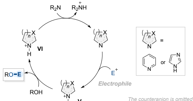
Scheme 23. General mechanism of N-Heterocycle-catalyzed alcohol functionalization.
