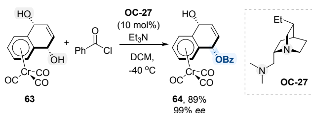
Scheme 37. Desymmetrization of meso -1,4-diol chromium complex.
