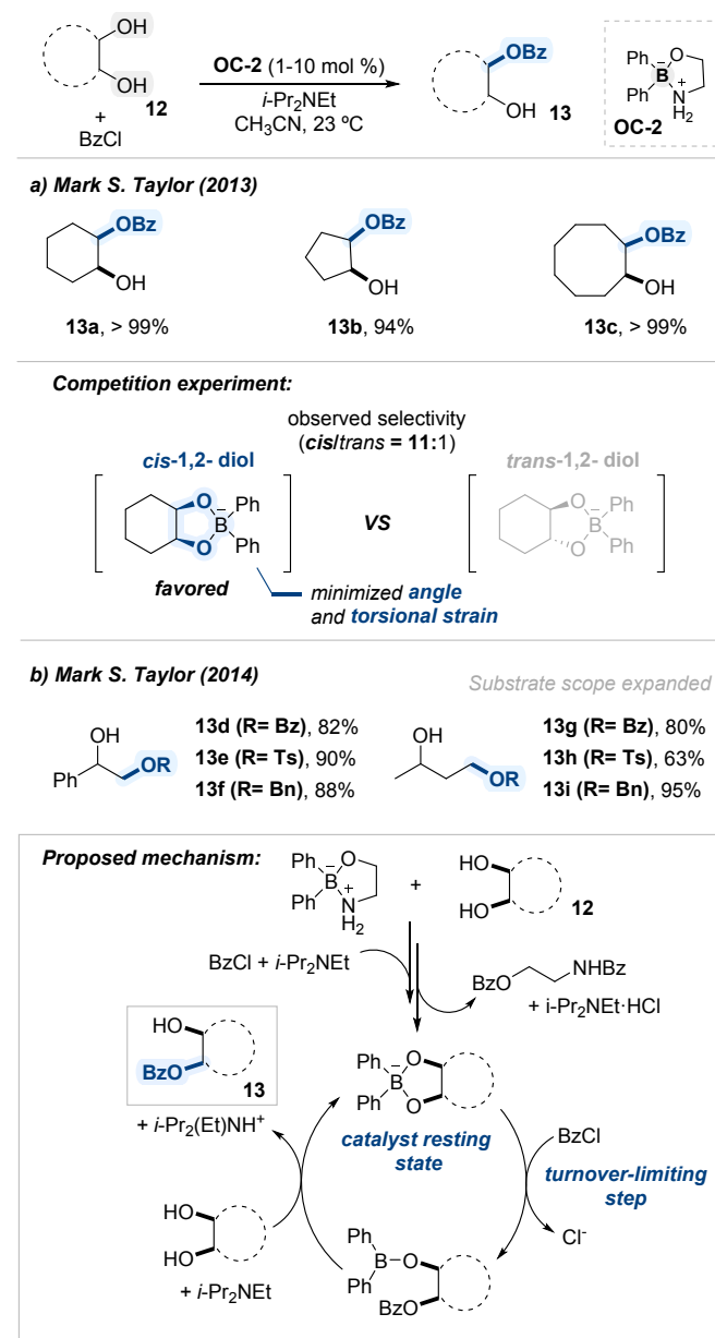
Scheme 9. Borinic acid-catalyzed regioselective acylation of diols.
