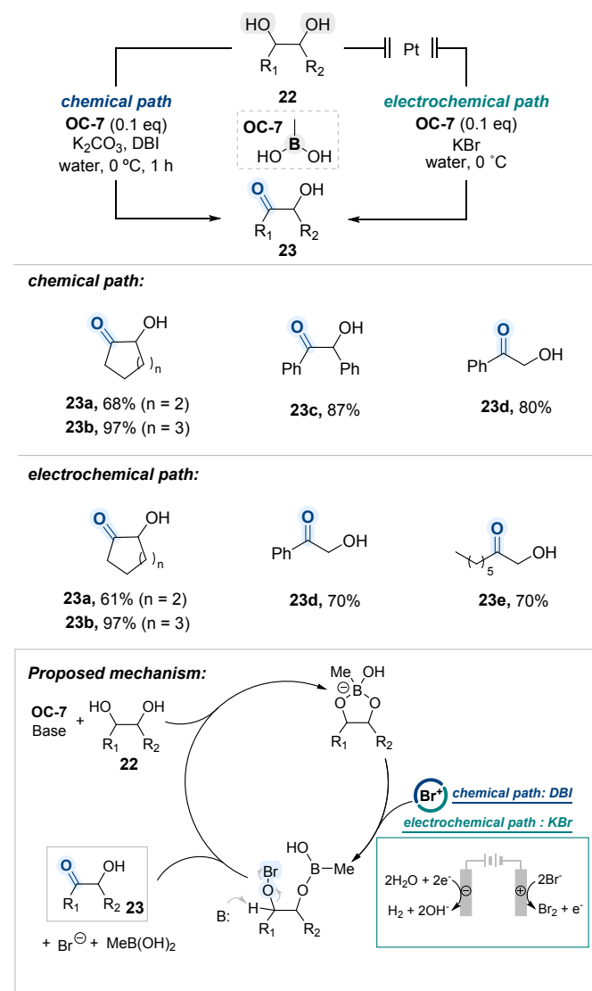
Scheme 15. Boronic acid-catalyzed selective oxidation of 1,2-diols to α-hydroxy ketones.
