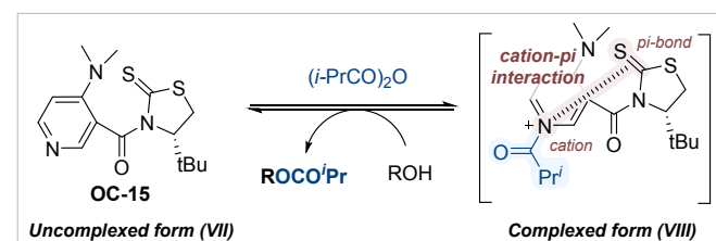
Scheme 25. Enantioselective isopropanoylation of meso -diols using chiral-DMAP catalyst (OC-15).
