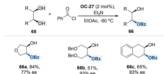
Scheme 38. Enantioselective benzoylation of meso -1,2-diols using cinchona alkaloid-derived catalyst ( OC-27 ).
