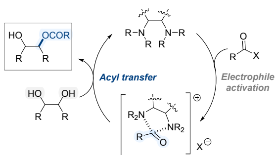
Schem 35. General mechanism of 1,2-diamine-catalyzed regioselective acylation of diols.
