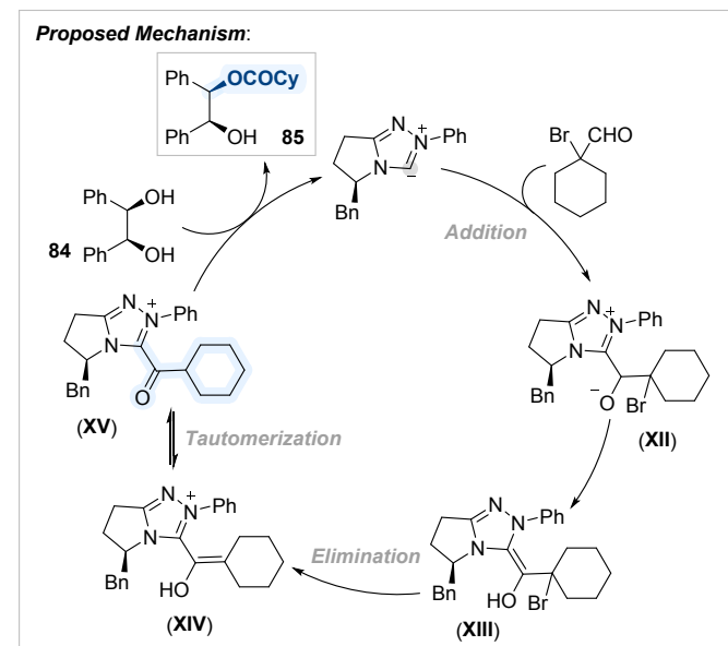
Scheme 48. Enantioselective acylation of meso -hydrobenzoin using chiral carbene catalyst ( OC-36 ).
