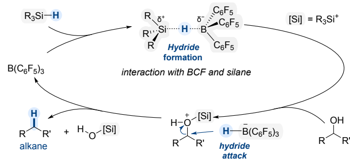
Scheme 2. General mechanism for BCF-catalysed deoxygenation of alcohols.
