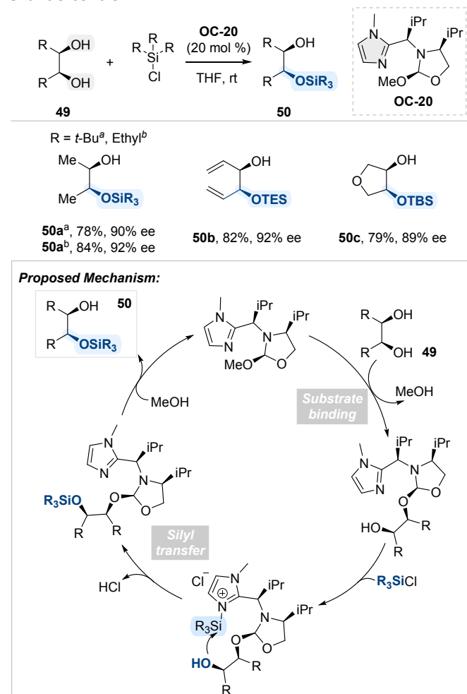
Scheme 27. Rotaxane-based catalyst ( OC-17 ) for asymmetric regioselective benzylation of meso -1,2-diol.
