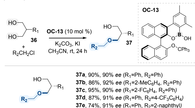
Scheme 20. Site-selective modification of diols catalyzed by OC-11 .
