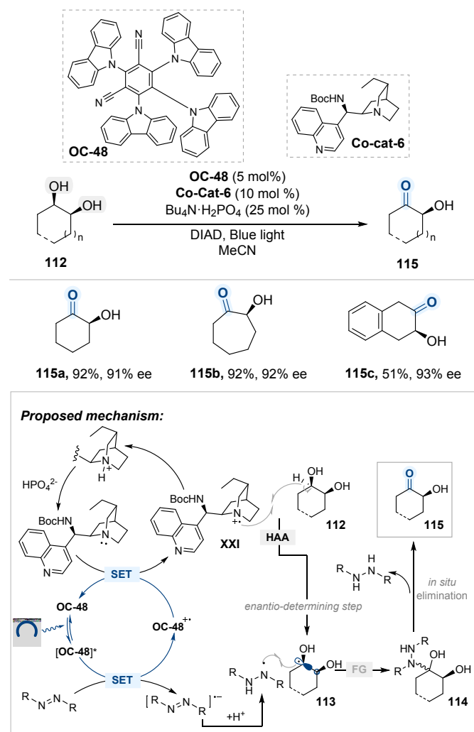
Scheme 60. Photocatalyzed oxidative desymmetrization of meso -1,2-diols.
