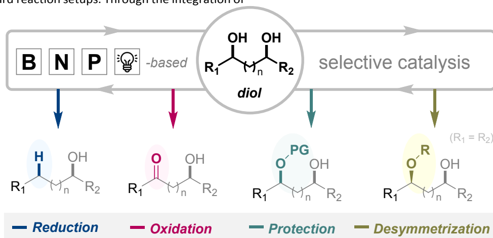
Figure 2. Selective functionalization of diol via organocatalysis.
