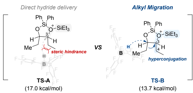
Scheme 4. BCF-catalyzed reductive pinacol-type rearrangement of internal 1,2-diols.
