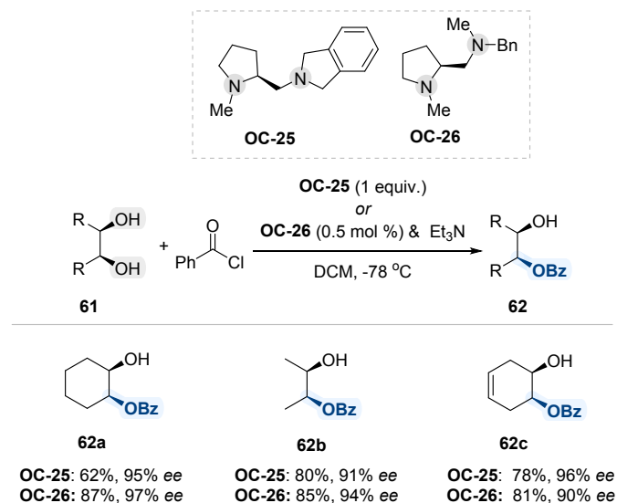
Scheme 36. Enantioselective benzoylation of meso -diol using chiral diamines ( OC-25 and OC-26 ).
