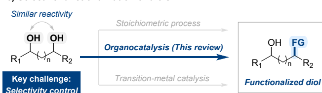
Figure 1. Overview of diol substrate: synthetic accessibility, pharmaceutical relevance, and the thematic focus of this review.
