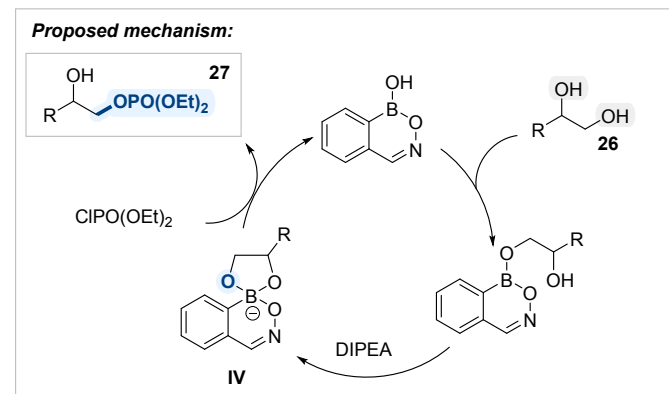
Scheme 18. Monophosphorylation reaction of vicinal diols catalyzed by benzoxazaborine scaffold.
