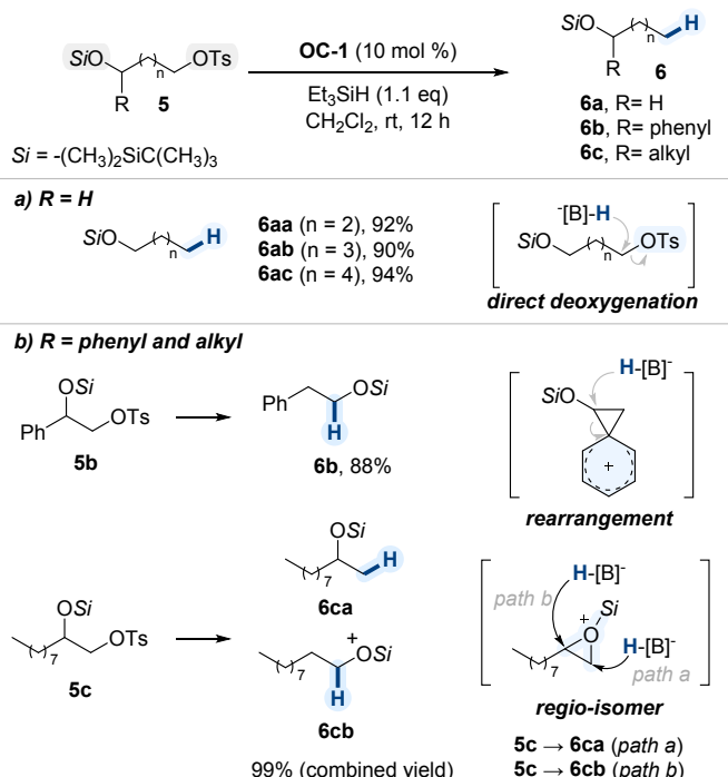
Scheme 5. Chemoselective deoxygenation of tosylated diols
