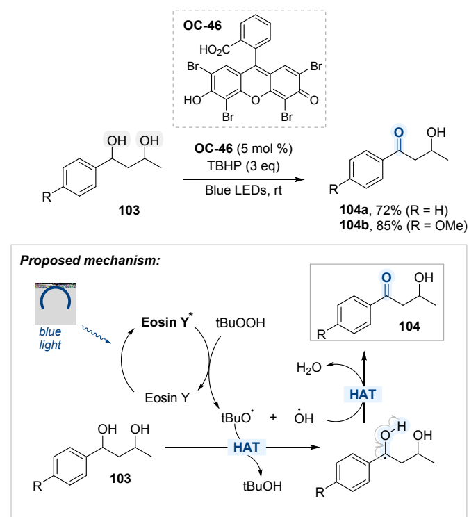
Scheme 57. Blue light-mediated chemoselective oxidation of 1,3-diol.
