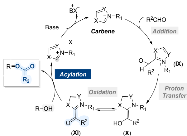
Scheme 47. General mechanism of NHC-catalyzed acylation of alcohols.
