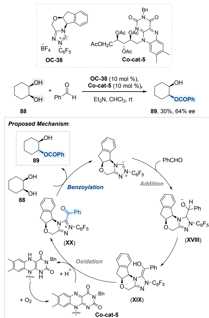
Scheme 50. Desymmetrization of 1,2-diol using chiral N -heterocyclic carbene ( OC-38 ) and a redox-active flavin ( Co-cat-5 ).
