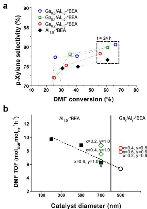
Fig. 4. (a) Reaction performance of Ga-impregnated catalysts, Ga_x/Al_{1.0} -*BEA, compared with the aluminosilicate control, Al_{1.0} -*BEA (black diamonds). Data above 50% conversion correspond to 24 h of reaction time. (b) DMF turnover frequency (TOF) within the first 3 h of reaction (see Table S6 of the ESI) for Al_{1.0} -*BEA catalysts (closed black squares) prepared with different sizes (where the 700 nm sample used as the control is highlighted with an asterisk), and Ga_xAl_y -*BEA catalysts from one-pot syntheses (open red circles). The open black circle is a hypothetical Al_{1.0} -*BEA sample of 900 nm size based on the extrapolated trendline (dashed line from linear regression). The Ga_x/Al_{1.0} -*BEA samples prepared by Ga impregnation are shown as open green diamonds.
