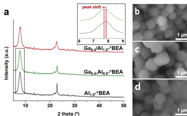
Fig. 1. (a) Powder XRD patterns of \text{Ga}_{0.4}/\text{Al}_{1.0}\text{-*BEA} , \text{Ga}_{0.4}\text{Al}_{0.6}\text{-*BEA} , and \text{Al}_{1.0}\text{-*BEA} (see also Fig. S1 of the ESI for other samples). Inset: example of the peak shift to lower 2\theta with isomorphic Ga substitution. (b – d) Scanning electron microscope (SEM) images of representative (b) \text{Ga}_{0.4}/\text{Al}_{1.0}\text{-*BEA} , (c) \text{Ga}_{0.4}\text{Al}_{0.6}\text{-*BEA} , and (d) \text{Al}_{1.0}\text{-*BEA} samples.
