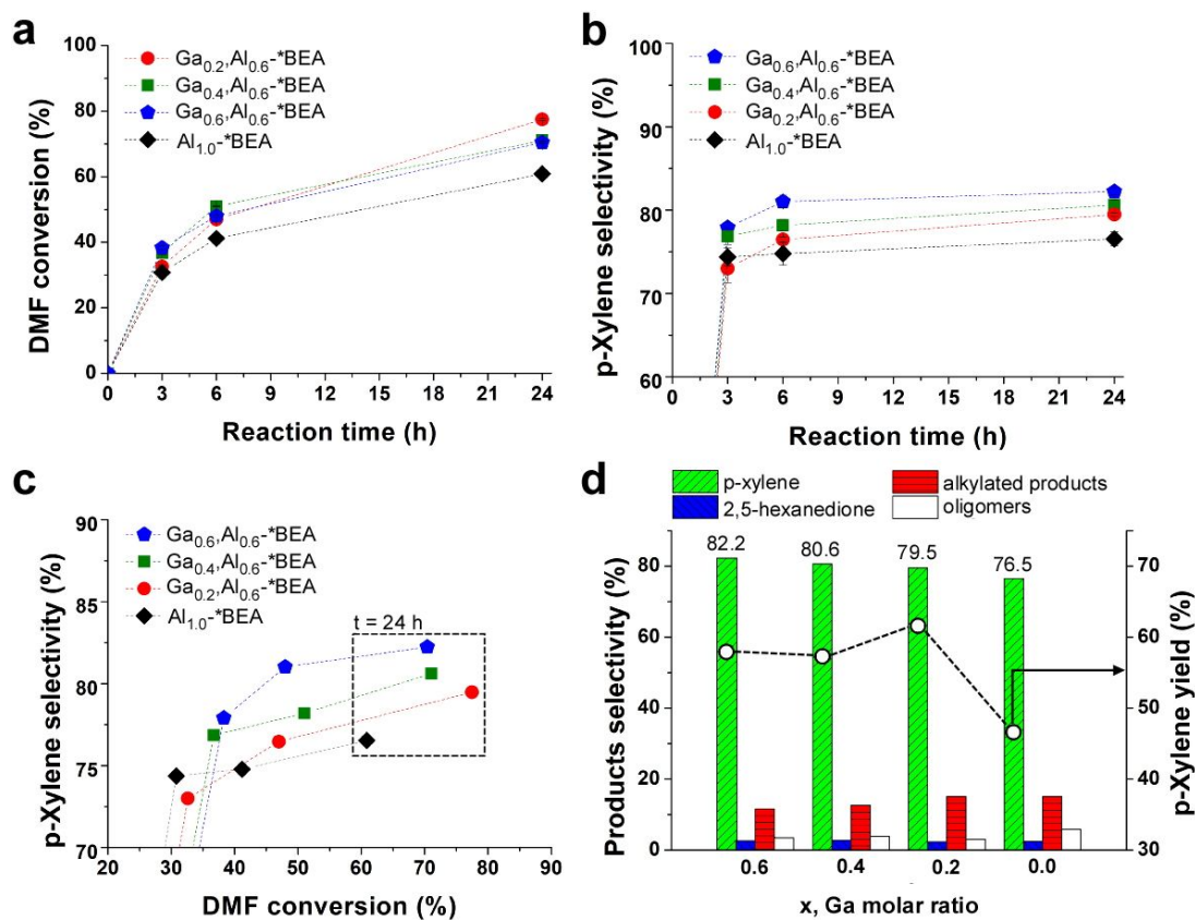
Fig. 3. Tandem Diels-Alder/dehydration reaction performance of *BEA catalysts at 250°C and 60 bar: (a) DMF conversion (starting from 0.23 M DMF in heptane) and (b) p-xylene selectivity vs reaction time; (c) p-xylene selectivity vs DMF conversion; and (d) products selectivities (histograms, left y-axis) and p-xylene yield (open circles, right y-axis) after 24 h of reaction. The x-axis lists the Ga molar ratio for each Ga x Al 0.6 -*BEA catalyst. Dashed lines are interpolated to guide the eye. Symbols are the average of three measurements for a single experiment. Error bars span two standard deviations (those not visible are less than the size of the symbol). This error is in good agreement with reproducibility tests that compared separate reactions in triplicate for the Al 1.0 -*BEA catalyst (see Fig. S10 of the ESI).
