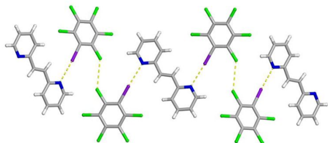
Fig. 2. X-ray structure of 2(\text{C}_6\text{I}_5\text{I}_7) \cdot (\text{2,2-BPE}) illustrating both the \text{I} \cdots \text{N} halogen bonds and Type I \text{Cl} \cdots \text{Cl} contacts to yield a wave-like one-dimensional chain. The \text{I} \cdots \text{N} halogen bonds and Type I \text{Cl} \cdots \text{Cl} contacts are shown with yellow dashed lines.
