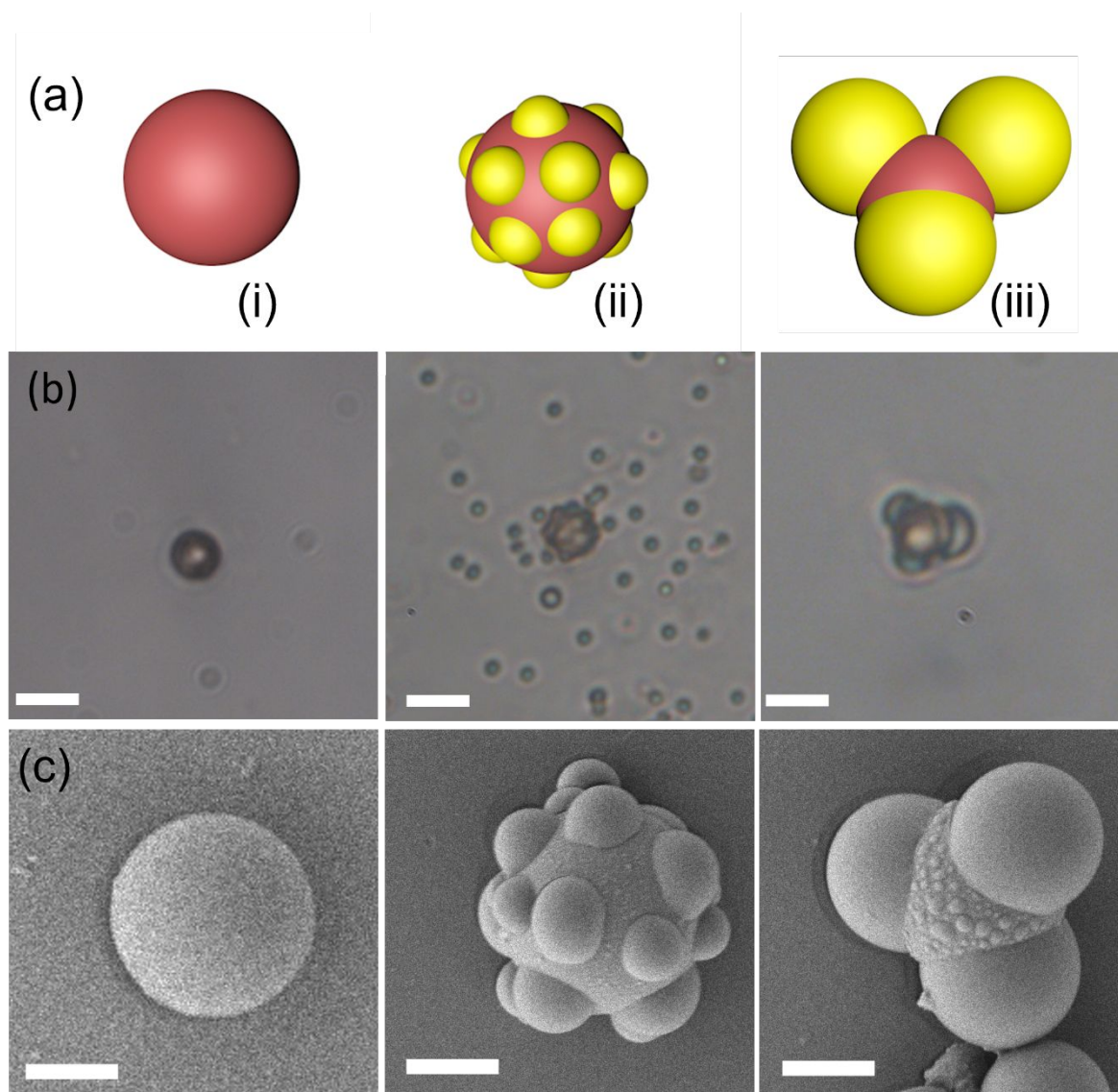
Fig. 2. Synthesis of three-lobed microrobots. (a) Scheme of synthesis (i) magnetic seed particles, (ii) heterogeneous nucleation of oil on the seeds, (iii) growth of droplets to achieve three lobes. (b) and (c) are corresponding respective optical and SEM images captured at different synthesis stages. Scale bars in (b) are 5 \mu\text{m} and in (c) are 2 \mu\text{m} .
