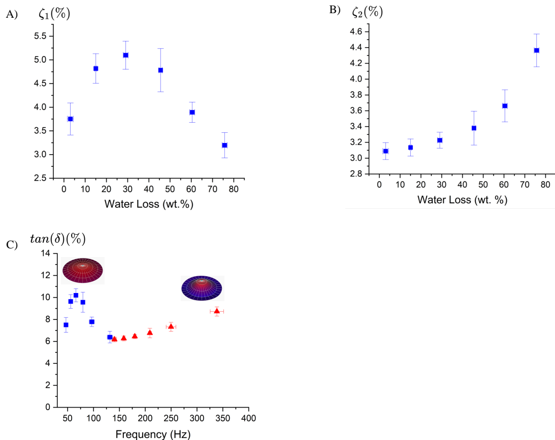
Figure 4: Evolution of damping ratios with water loss: A) \zeta_1 ; B) \zeta_2 ; C) Loss tangent vs Frequency.
