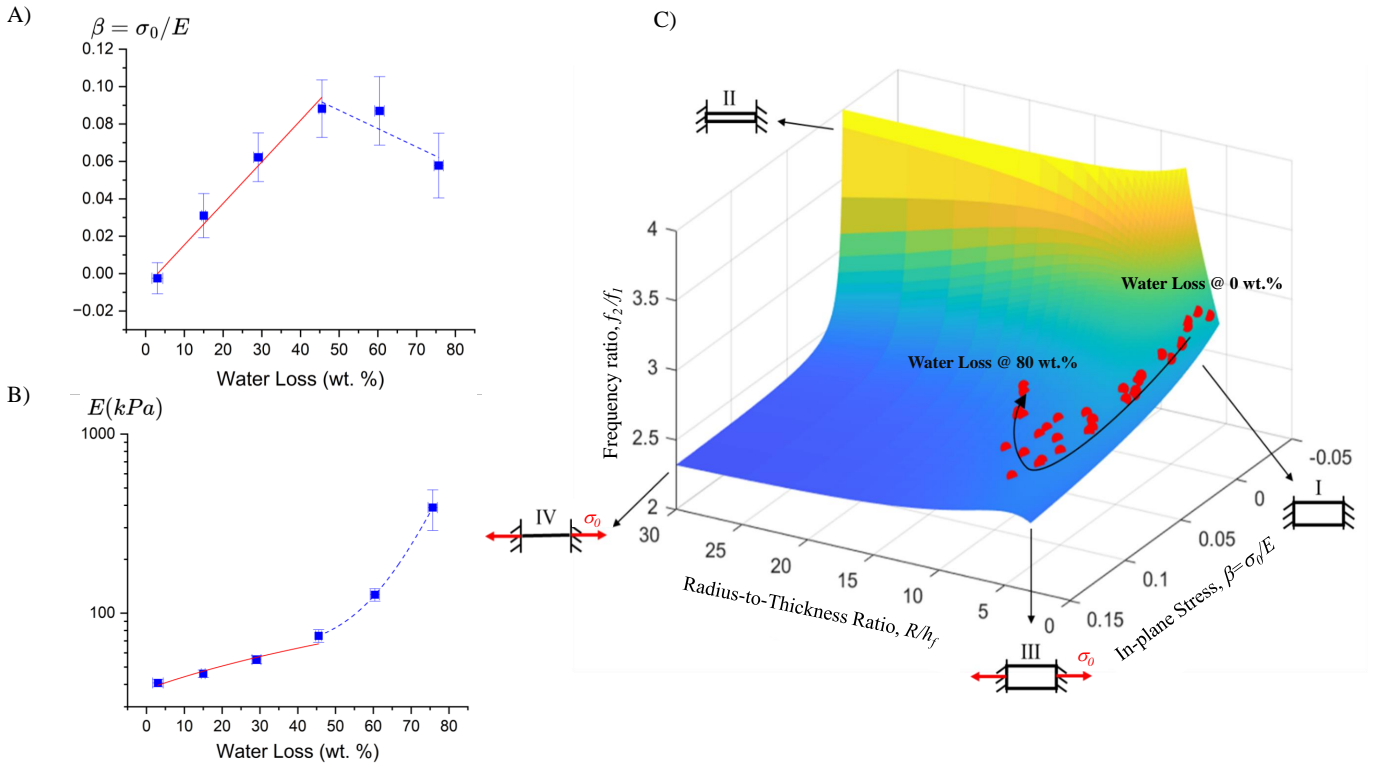
Figure 3: A) Evolution of normalized in-plane stress \beta = \sigma_0/E with water loss; B) Evolution of estimated elastic modulus E with water loss, and C) Frequency ratio as a function of normalized in-plane stress and radius-to-thickness ratio. Markers in C) correspond to the experimental data. Inset sketches in C) illustrate four extreme conditions for the disks. Arrow in C) indicates increasing water loss. The dashed curves denote the regression analysis
