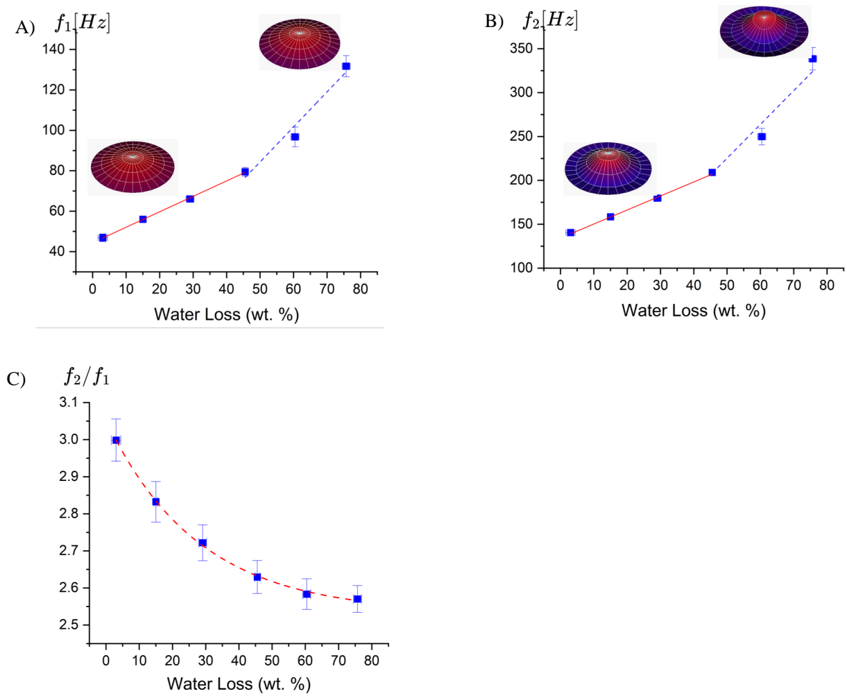
Figure 2: Evolution of modal frequencies with water loss: A) First mode frequency f_1 ; B) Second mode frequency f_2 , and C) Frequency ratio f_2/f_1 . The dashed curves denote the regression analysis
