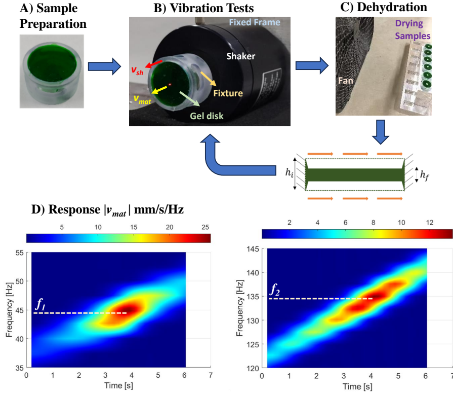
Figure 1: Experimental details: A) Gelatin preparation and curing to a fixture; B) Components in vibration testing; C) Dehydration process, and D) Representative time-frequency-amplitude plots of the material response |v_{mat}| around mode 1 and mode 2 as processed from frequency sweep data.
