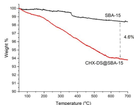
Fig. 7 TGA analysis of as-synthesized SBA-15 and CHX-DS@SBA-15.
