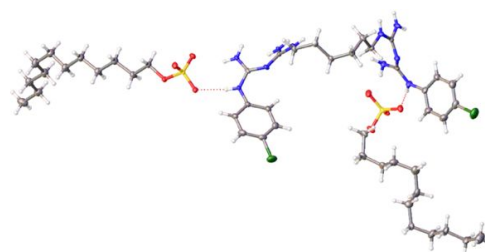
Fig. 2 Structure of CHX complexing with two SDS units.
