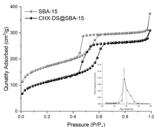
Fig. 8 Nitrogen (77 K) sorption isotherms of calcined SBA-15 and CHX-DS@SBA-15. Pore size distribution shown in inset.
